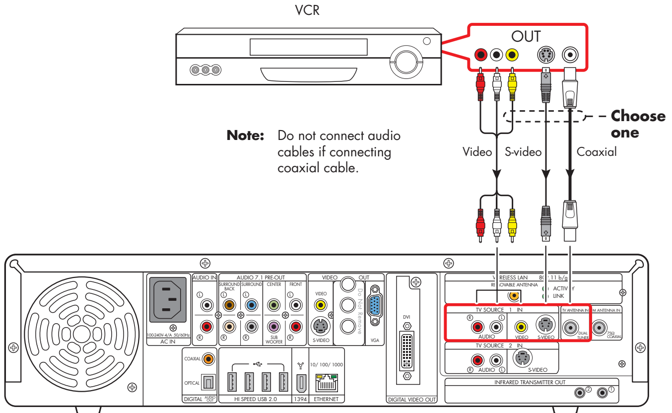
VCR connection
